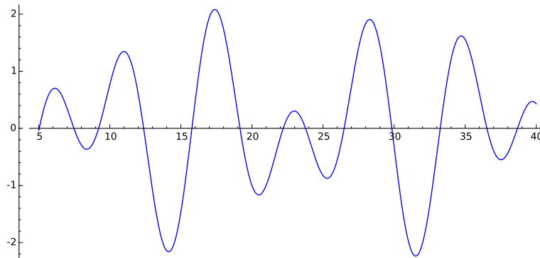
Figure 32.2: Plot of \hat{\Phi}_{\leq 3}(\theta)
