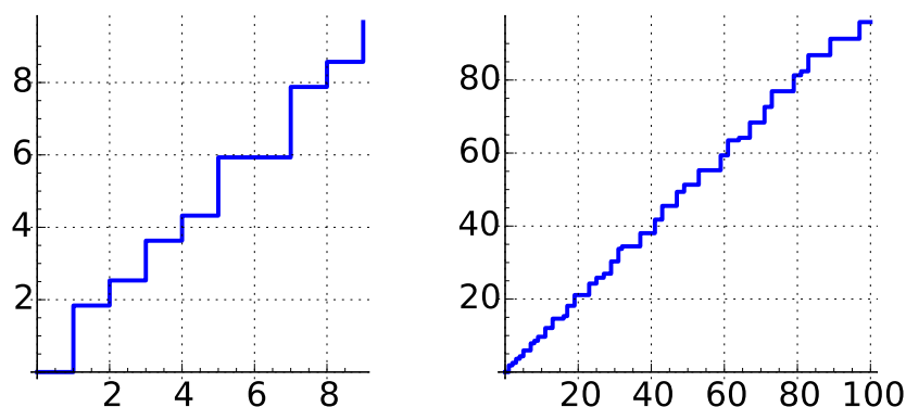
Figure 19.1: The newly constructed staircase that counts tprime powers
