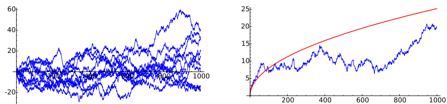
Figure 12.2: Ten Random Walks
