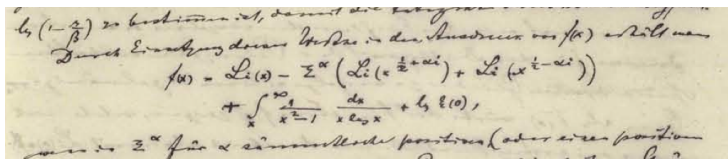
Figure 36.5: Riemann analytic formula for \pi(X) .
