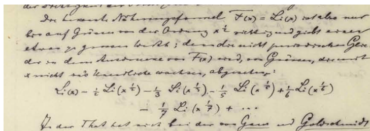
Figure 36.2: Riemann defining R(X) in his manuscript
