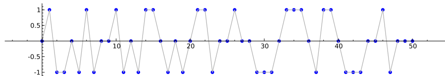
Figure 36.1: The blue dots plot the values of the Moebius function \mu(n) , which is only defined at integers.
