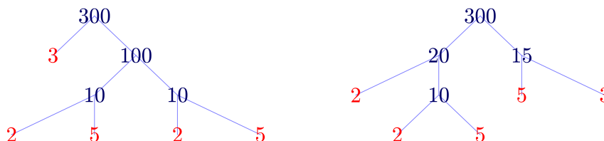
Figure 2.2: Factor trees that illustrates the factorization of 300 as a product of primes.
