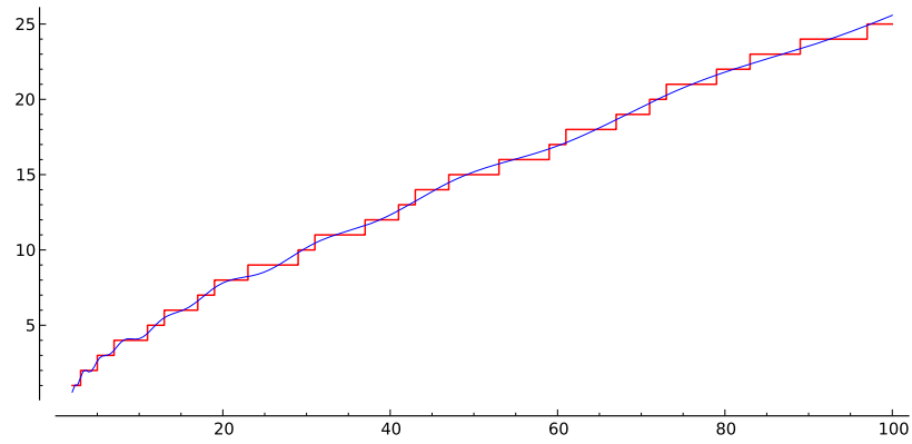
Figure 36.6: The function R_1 approximating the staircase of primes up to 100
