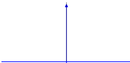
Figure 26.3: The Dirac \delta -“function” (actually distribution), where we draw a vertical arrow to illustrate the delta function with support at a given point.
