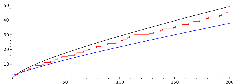
Figure 13.1: Plots of \text{Li}(X) (top), \pi(X) (in the middle), and X/\log(X) (bottom).
