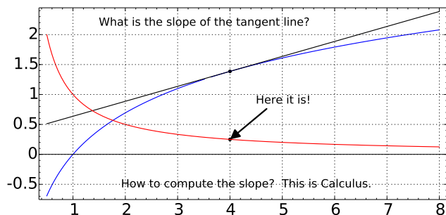
Figure 25.3: Calculus
