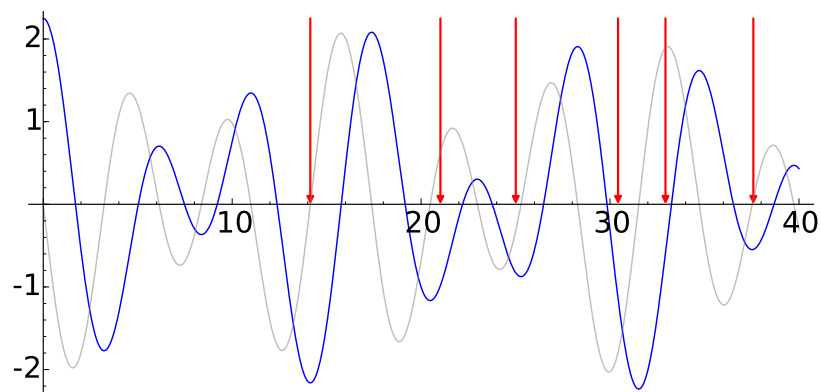
Figure 32.4: \hat{\Phi}_{\leq 3}(\theta)
