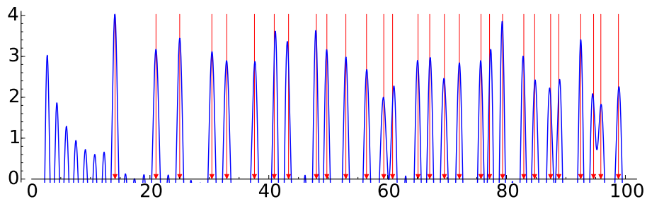
Figure 30.4: Plot of -\sum_{p^n \leq 50} \frac{\log(p)}{p^{n/2}} \cos(t \log(p^n)) with arrows pointing to the spectrum of the primes
