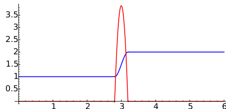
Figure 25.7: Second picture of the derivative of a smooth approximation to a function that jumps.
