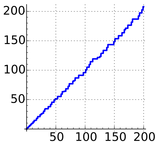
Figure 38.6: Illustration of the staircase \psi(X) constructed in Chapter 19 that counts weighted prime powers.
