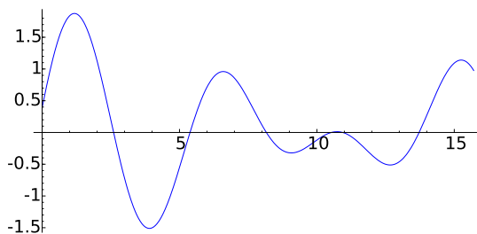
Figure 20.4: Graph of two “sine” waves with different phase.
