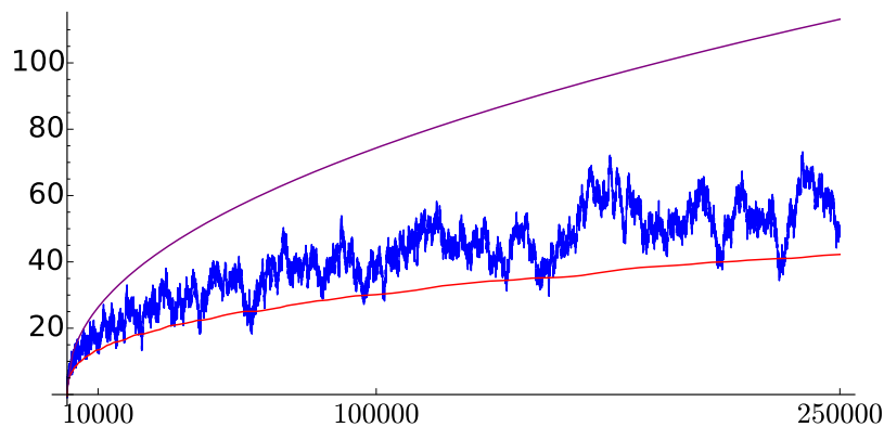
Figure 16.1: \text{Li}(X) - \pi(X) (blue middle), its Césaro smoothing (red bottom), and \sqrt{\frac{2}{\pi}} \cdot \sqrt{X/\log(X)} (top), all for X \leq 250,000
