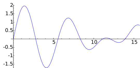
Figure 20.3: Graph of Sum of the Two Sine Waves with Different Frequencies
