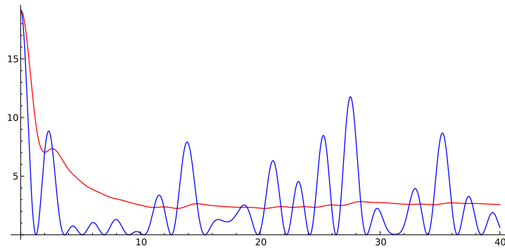
Figure 15.2: The red plot is the Césaro smoothing of the blue plot
