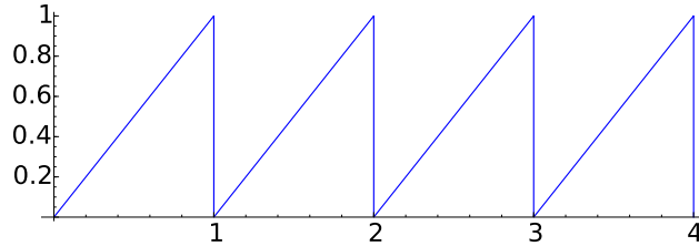
Figure 20.10: Graph of Sawtooth Wave
