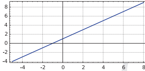
Figure 25.2. Graph of the function f(a) = a + 1
