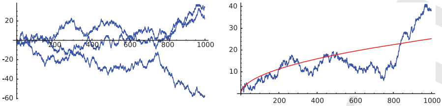
Figure 12.1. Three Random Walks
