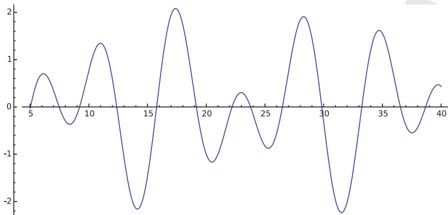
Figure 32.2. Plot of \hat{\Phi}_{\leq 3}(\theta)
