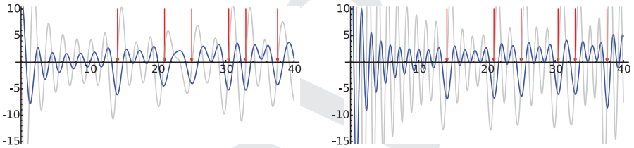
Figure 32.6. Plot of \hat{\Phi}_{\leq C}(\theta) for C = 10 and 100
