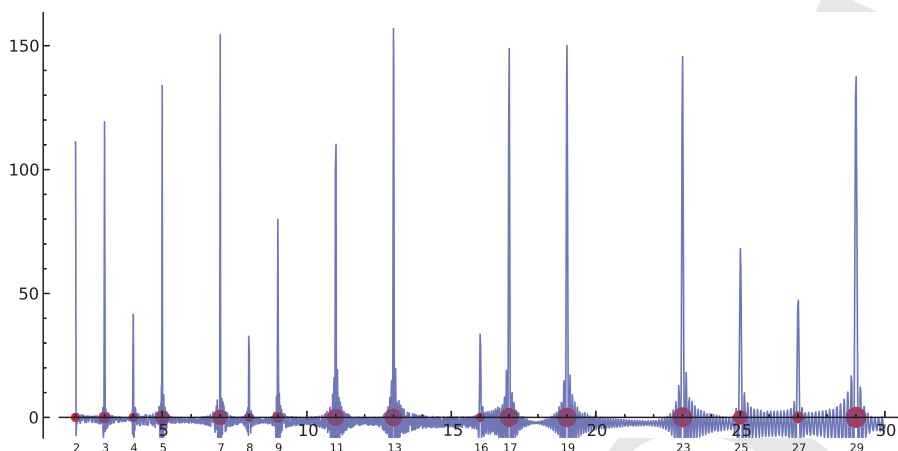
Figure 30.6. Illustration of -\sum_{i=1}^{1000} \cos(\log(s)\theta_i) , where \theta_1 \sim 14.13, \dots are the first 1000 contributions to the spectrum. The red dots are at the prime powers p^n , whose size is proportional to \log(p)
