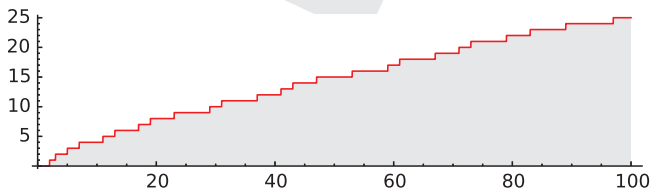
Figure 7.10. Staircase of primes up to 100
