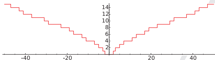
Figure 27.2. Even extension of the staircase of primes
