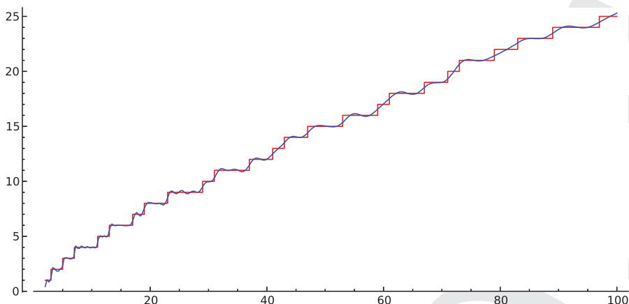
Figure 36.8. The function R_{25} approximating the staircase of primes up to 100
