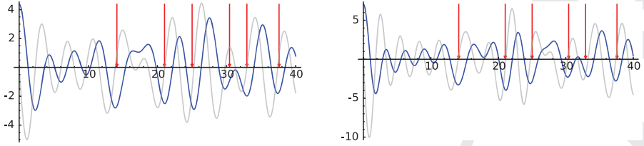
Figure 32.5. Plot of \hat{\Phi}_{\leq C}(\theta) for C = 5 and 10
