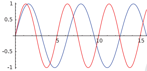
Figure 20.2. Graph of two sine waves with different frequencies
