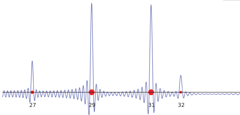
Figure 35.2. Illustration of -\sum_{i=1}^{1000} \cos(\log(s)\theta_i) in the neighborhood of a twin prime. Notice how the two primes 29 and 31 are separated out by the Fourier series, and how the prime powers 3^3 and 2^5 also appear
