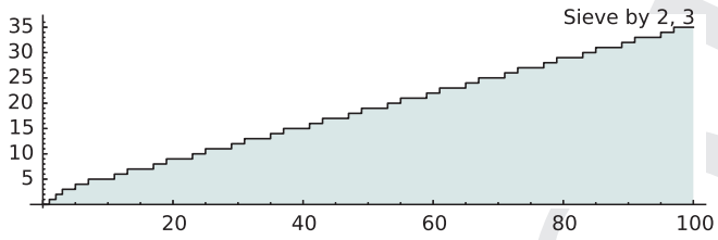
Figure 7.7. Sieving out multiples of 2 and 3
