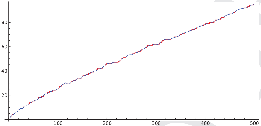
Figure 36.10. The function R_{50} approximating the staircase of primes up to 500
