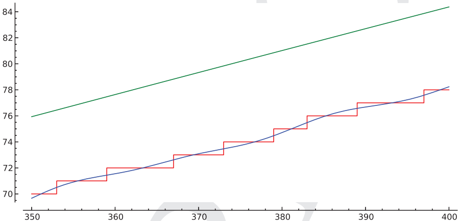
Figure 36.11. The function \text{Li}(X) (top, green), the function R_{50}(X) (in blue), and the staircase of primes on the interval from 350 to 400
