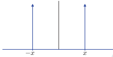
Figure 29.1. The sum (\delta_x(t) + \delta_{-x}(t))/2 , where we draw vertical arrows to illustrate the Dirac delta functions
