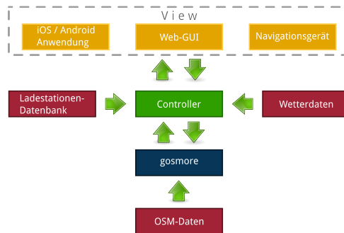
Abbildung 1: Architecture
