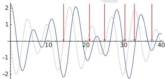
Figure 32.4. \hat{\Phi}_{\leq 3}(\theta)
