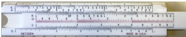
Figure 10.4: A slide rule computes 2X by using that \log(2X) = \log(2) + \log(X)
