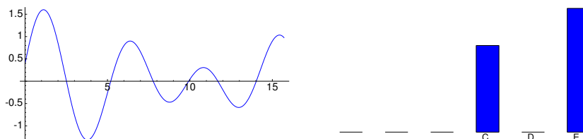
Figure 20.9: Spectral picture of a CE chord
