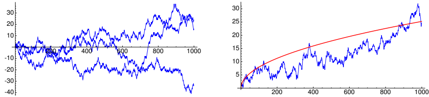
Figure 12.1: Three Random Walks
