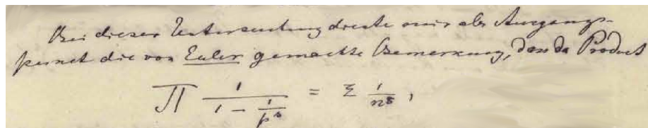
Figure 17.3: From a manuscript of Riemann’s 1859 paper written by a contemporary of Riemann (possibly the mathematician Alfred Clebsch).
