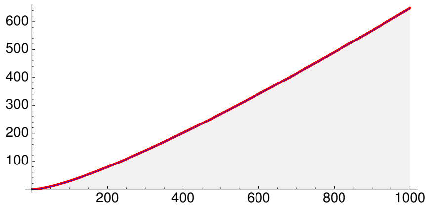
Figure 33.3: The staircase of the Riemann spectrum looks like a smooth curve
