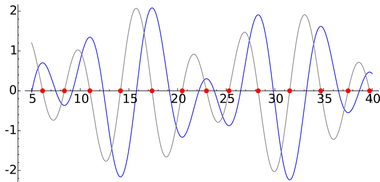
Figure 32.3: Plot of \hat{\Phi}_{\leq 3}(\theta) in blue and its derivative in grey
