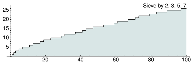
Figure 7.8: Sieving out multiples of 2, 3, 5, and 7.
