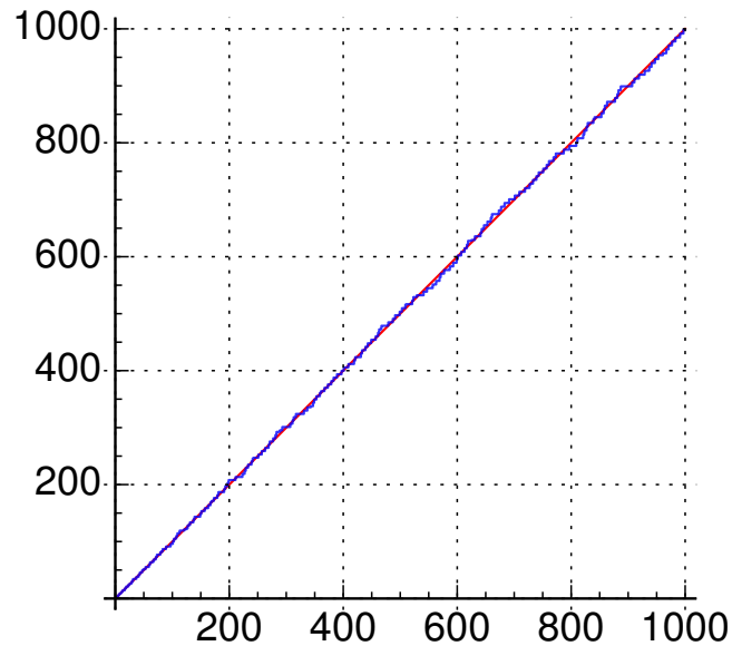
Figure 19.2: The newly constructed staircase is close to the 45 degree line.
