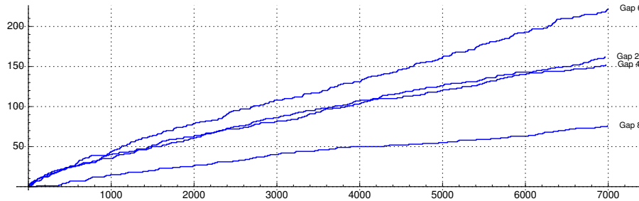
Figure 6.2: Plots of \text{Gap}_k(X) for k = 2, 4, 6, 8 . Which wins?
