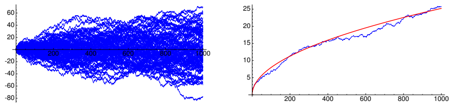
Figure 12.3: One Hundred Random Walks
