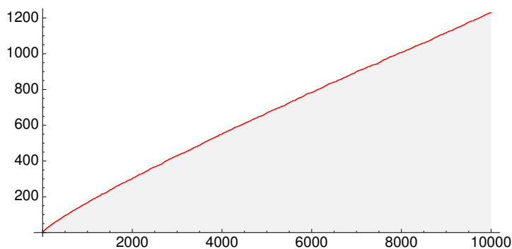
Figure 8.2: Staircases of primes up to 10,000
