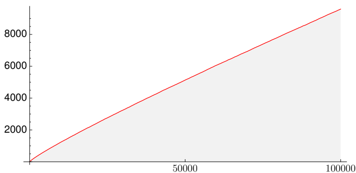
Figure 8.3: Primes up to 100,000.
