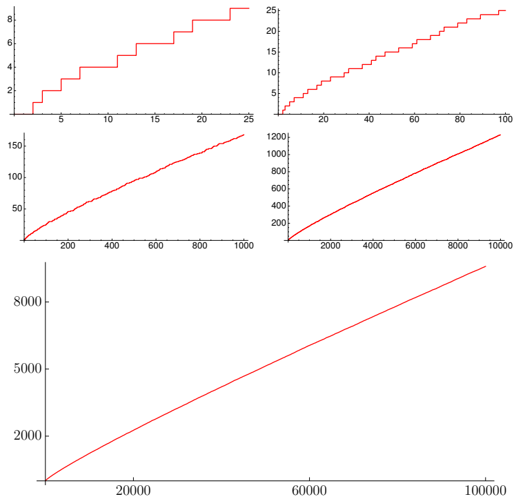
Figure 18.1: The Staircase of Primes
