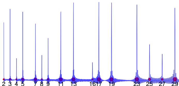
Figure 30.6: Illustration of -\sum_{i=1}^{1000} \cos(\log(s)\theta_i) , where \theta_1 \sim 14.13, \dots are the first 1000 contributions to the spectrum. The red dots are at the prime powers p^n , whose size is proportional to \log(p) .
