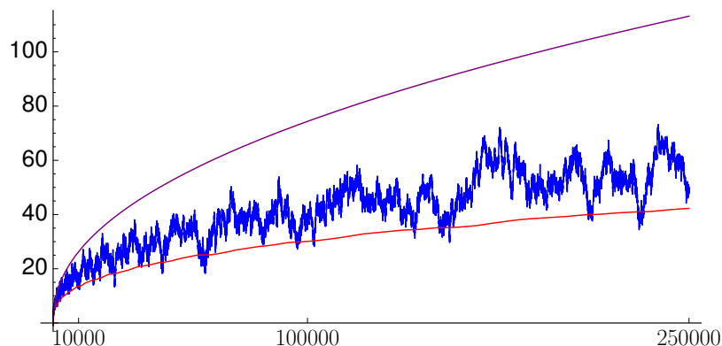
Figure 16.1: \text{Li}(X) - \pi(X) (blue middle), its Cesàro smoothing (red bottom), and \sqrt{\frac{2}{\pi}} \cdot \sqrt{X/\log(X)} (top), all for X \leq 250,000
