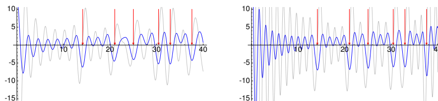
Figure 32.6: Plot of \hat{\Phi}_{\leq C}(\theta) for C = 10 and 100
