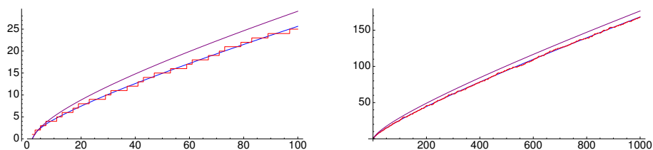
Figure 36.3: Comparisons of \text{Li}(X) (top), \pi(X) (middle), and R(X) (bottom, computed using 100 terms)
