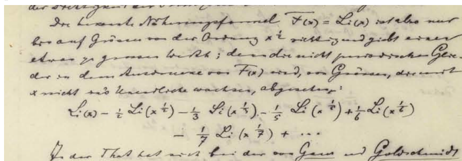
Figure 36.1: Riemann defining R(X) in his manuscript
