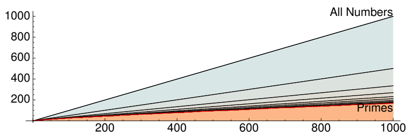
Figure 7.6: Sieving for primes up to 1000
