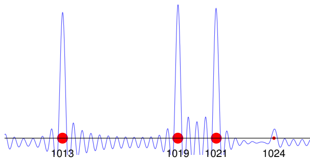
Figure 35.3: Fourier series from 1,000 to 1,030 using 15,000 of the numbers \theta_i . Note the twin primes 1,019 and 1,021 and that 1,024 = 2^{10} .
