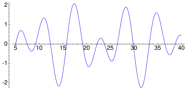
Figure 32.2: Plot of \hat{\Phi}_{\leq 3}(\theta)
