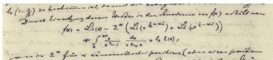
Figure 36.5: Riemann's analytic formula for \pi(X)
