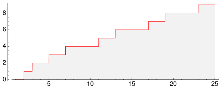
Figure 7.9: Staircase of primes up to 25
