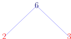
Figure 2.1: The number 6 = 2 \times 3
