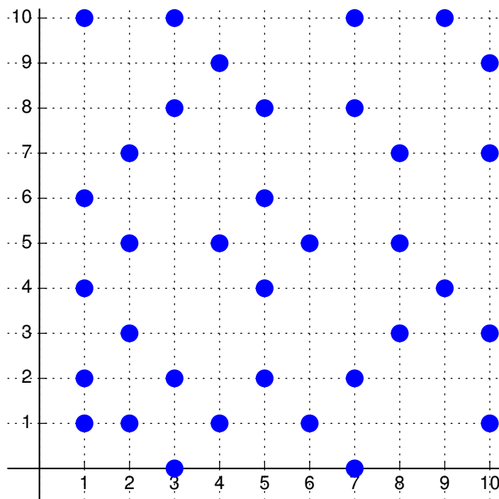
Figure 38.1: Gaussian primes with coordinates up to 10
