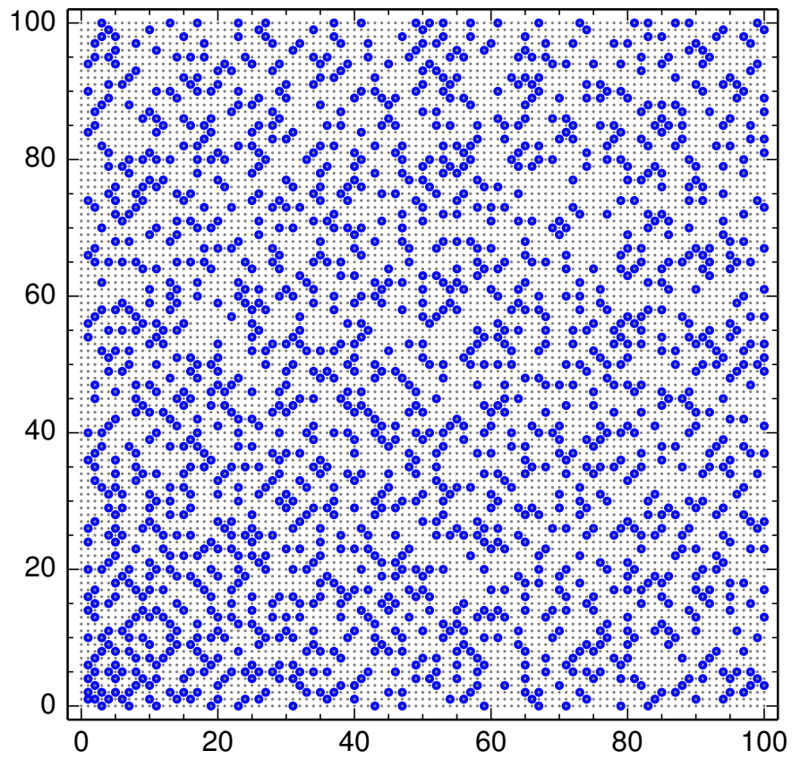
Figure 38.2: Gaussian primes with coordinates up to 100
