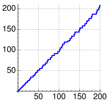
Figure 39.2: Illustration of the staircase \psi(X) constructed in Chapter 19 that counts weighted prime powers.
