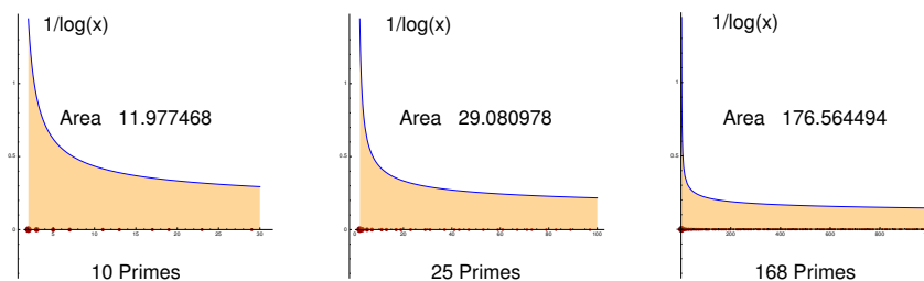
Figure 10.6: The expected tally of the number of primes \leq X is approximated by the area underneath the graph of 1/\log(X) from 1 to X .
