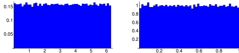
Figure 34.1: Frequency histogram of Odlyzko's computation of the Riemann spectrum modulo 2\pi (left) and modulo 1 (right)
