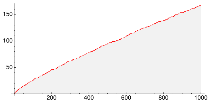
Figure 8.1: Staircases of primes up to 1,000
