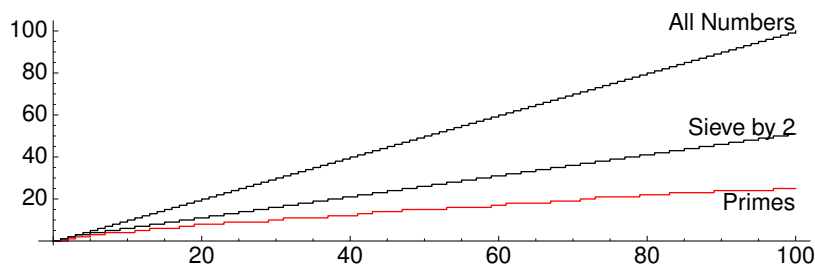
Figure 7.5: Sieving by removing multiples of 2 up to 100
