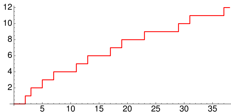
Figure 31.2: Prime numbers up to 37
