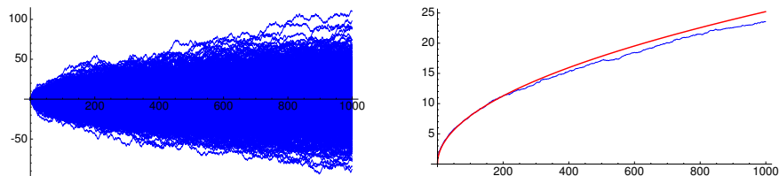
Figure 12.4: One Thousand Random Walks
