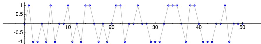
Figure 36.2: The blue dots plot the values of the Möbius function \mu(n) , which is only defined at integers.
