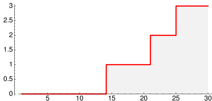
Figure 33.1: The staircase of the Riemann spectrum
