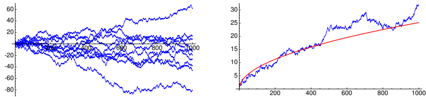
Figure 12.2: Ten Random Walks
