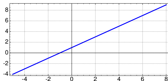
Figure 25.2: Graph of the function f(a) = a + 1
