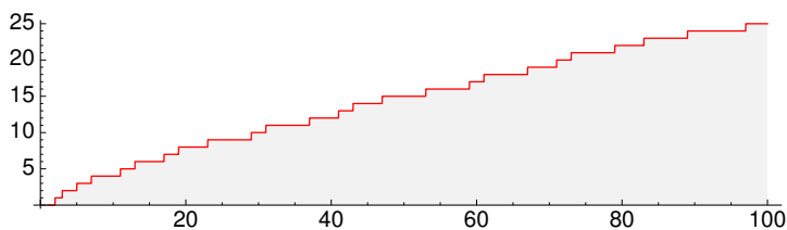
Figure 7.10: Staircase of primes up to 100
