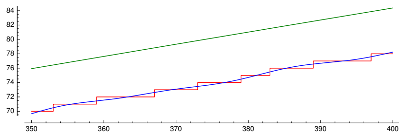
Figure 36.11: The function \text{Li}(X) (top, green), the function R_{50}(X) (in blue), and the staircase of primes on the interval from 350 to 400.
