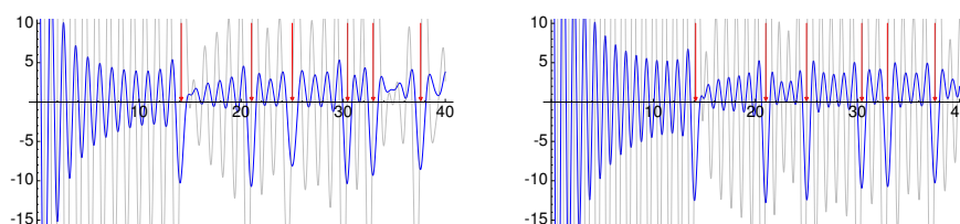
Figure 32.7: Plot of \hat{\Phi}_{\leq C}(\theta) for C = 200 and 500
