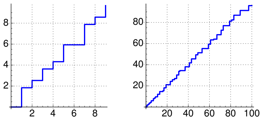
Figure 19.1: The newly constructed staircase that counts prime powers
