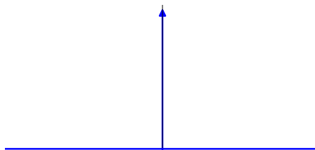
Figure 26.3: The Dirac \delta -“function” (actually distribution), where we draw a vertical arrow to illustrate the delta function with support at a given point.
