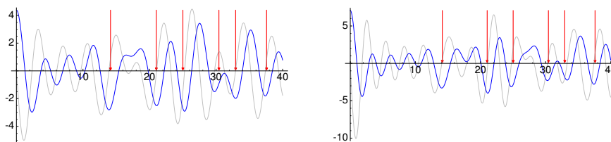
Figure 32.5: Plot of \hat{\Phi}_{\leq C}(\theta) for C = 5 and 10
