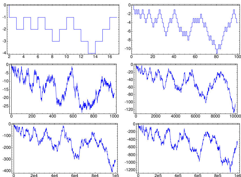
Figure 6.3: Racing Multiplicatively Even and Odd Numbers.
